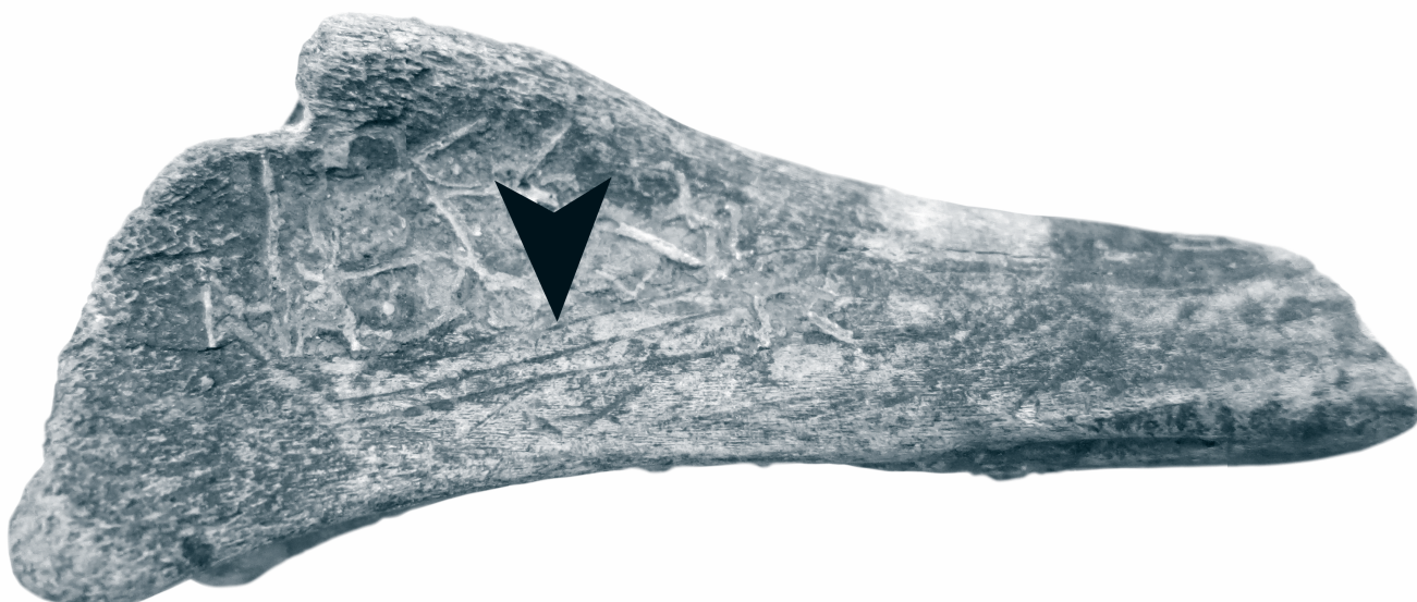
Text-fig. 11. Longitudinal defleshing marks on ochre-stained tibia 98-601a-F to extract the meat of m. fibularis longus and part of m. flexor digitorum , fossilised rootlets visible on the shaft.
