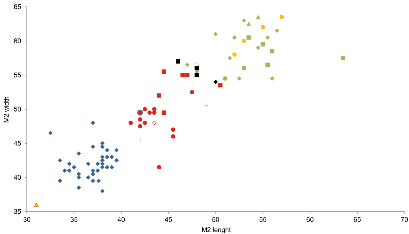
Text-fig. A2. Scatter diagram of M2 sizes of different species of Prosantorhinus and Diaceratherium .
