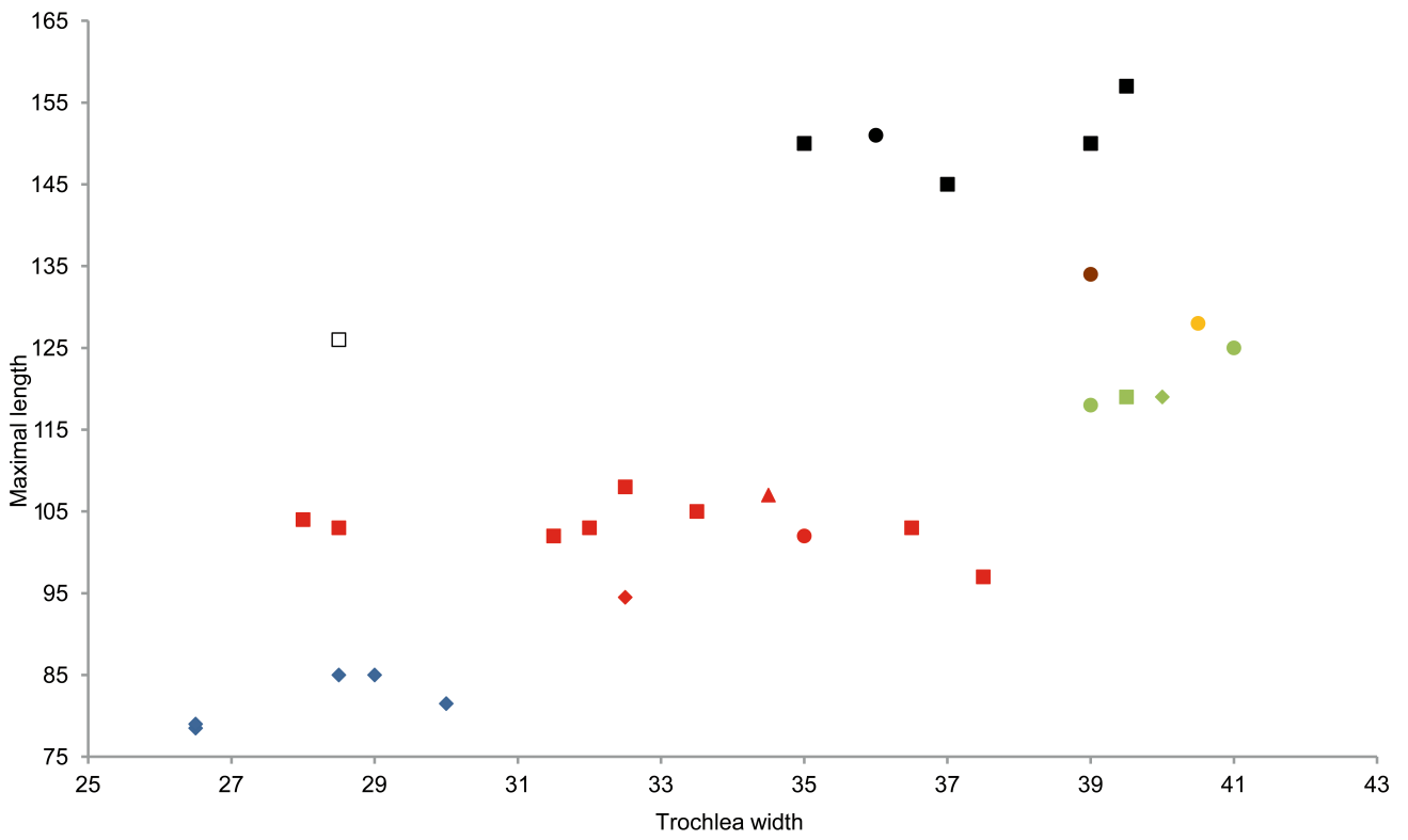
Text-fig. A3. Scatter diagram of the size of MC II of Prosantorhinus and Diaceratherium .
