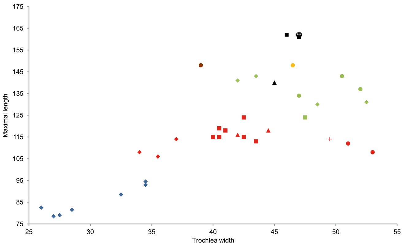
Text-fig. A4. Scatter diagram of the size of MC III of Prosantorhinus and Diaceratherium .
