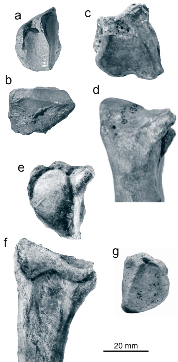
Text-fig. 2. Metatarsal II of different species of Prosantorhinus . a, b. Prosantorhinus douvillei , Montréal-du-Gers, left MT II, a. proximal view, b. lateral view; c, d. Prosantorhinus germanicus , Sandelzhausen, left MT II, c. proximal view, d. lateral view; e, f. Prosantorhinus laubei , Ahnikov, left MT II, e. proximal view, f. lateral view; g. Prosantorhinus aurelianensis , Rothenstein 16, juvenile, right MT II, proximal view.
