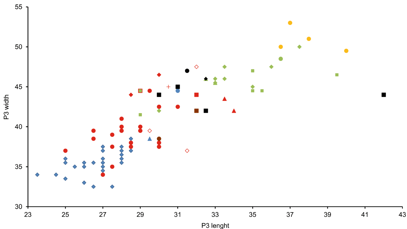
Text-fig. A1. Scatter diagram of P3 sizes of different species of Prosantorhinus and Diaceratherium .
