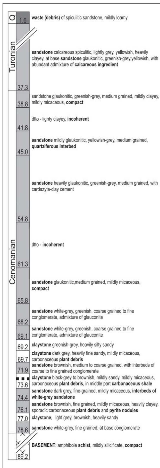
Text-fig. 3. Simplified log of borehole VMK-151, drilled near Maletín, showing major stratigraphic units of studied area.
